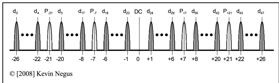
Figure 6 OFDM subcarriers for IEEE 802.11a
