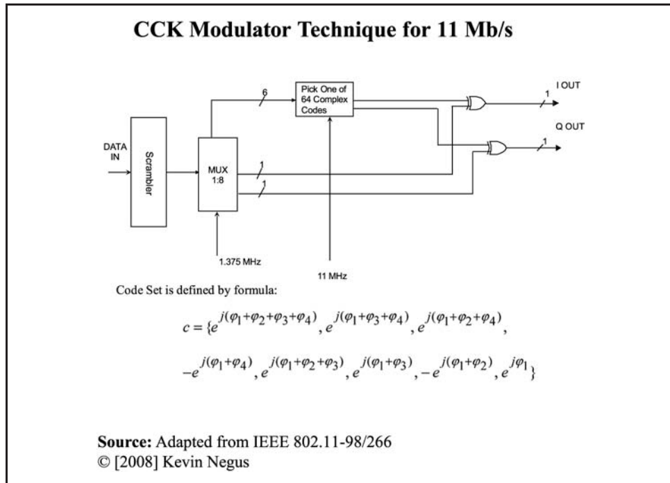
Figure 8 802.11b Modulator block diagram
