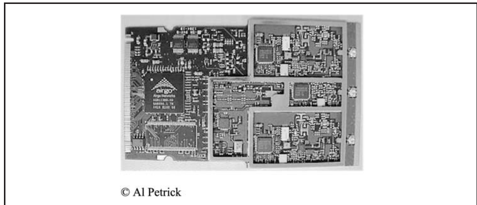
Figure 12 Airgo 802.11 “pre-N” MIMO reference design
