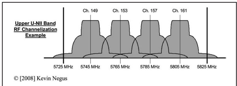
Figure 7 OFDM channelization for IEEE 802.11a
