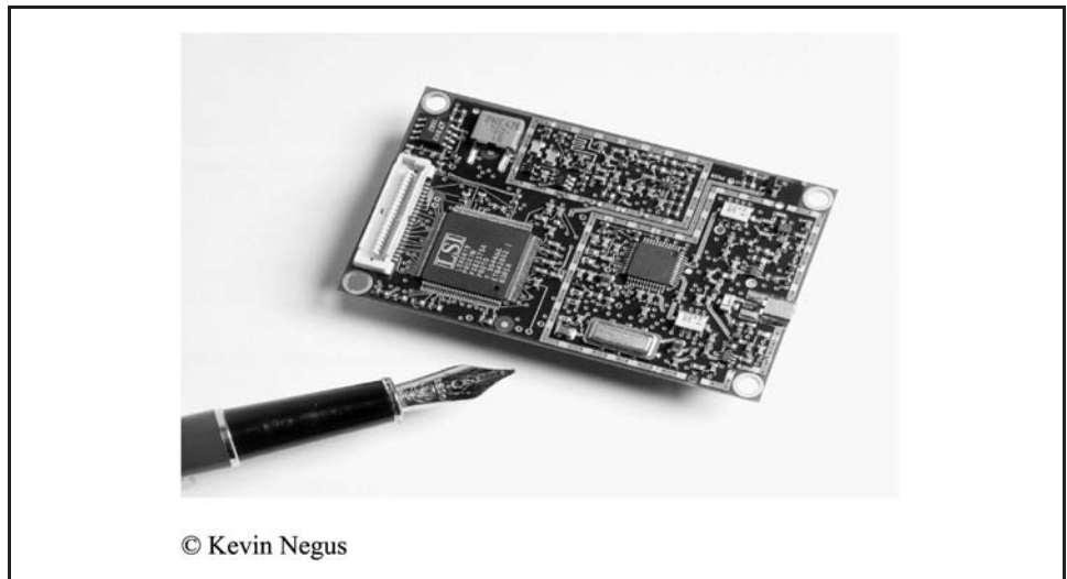
Figure 5 HomeRF “two-chip” adaptor, circa 1998
