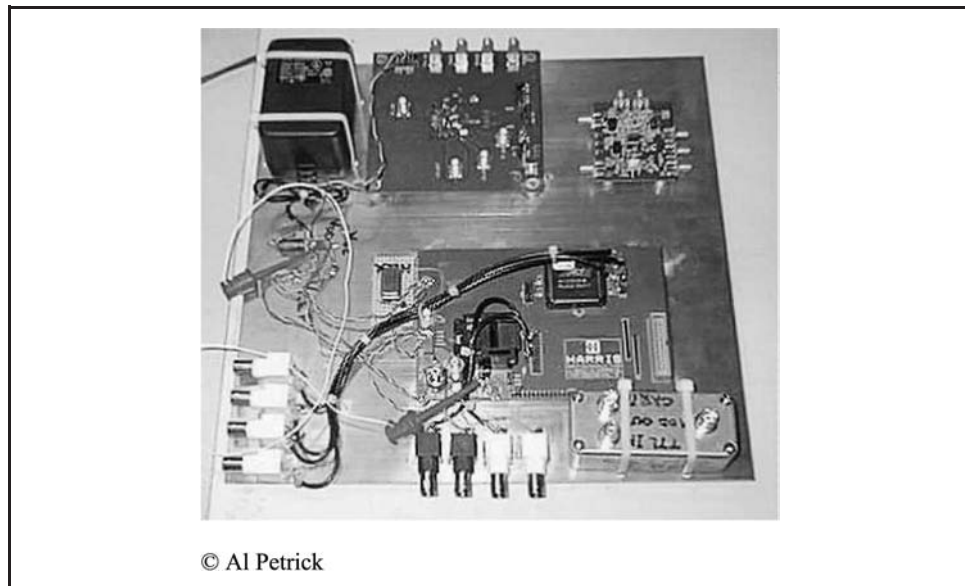
Figure 9 Harris PRISM 802.11b Chipset, circa 1998
