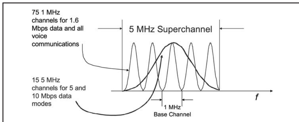
Figure 10 HomeRF 2.0 channelization
