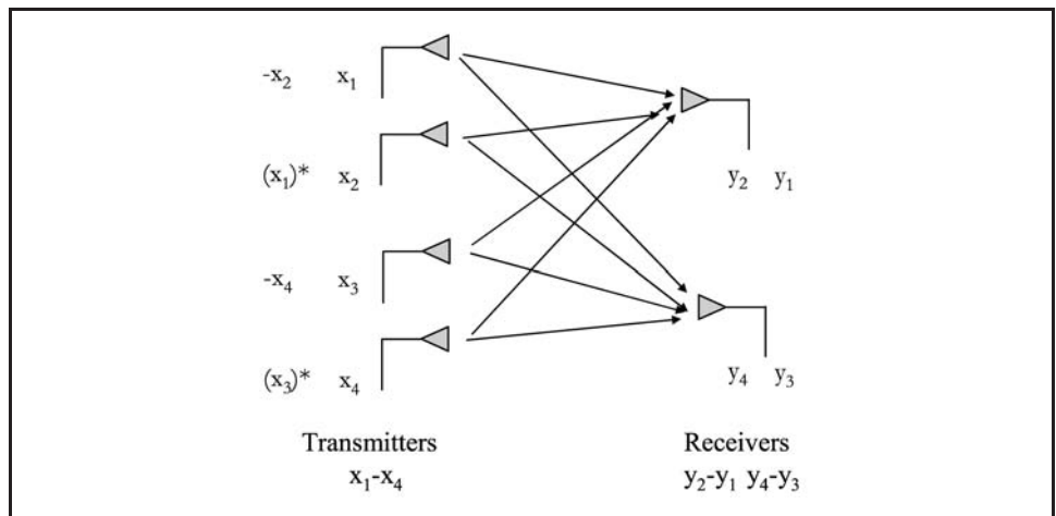
Figure 11 MIMO and spatial division multiplexing
