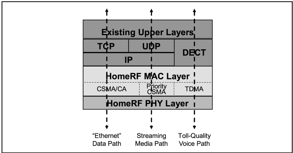
Figure 4 Hybrid MAC processing in HomeRF
